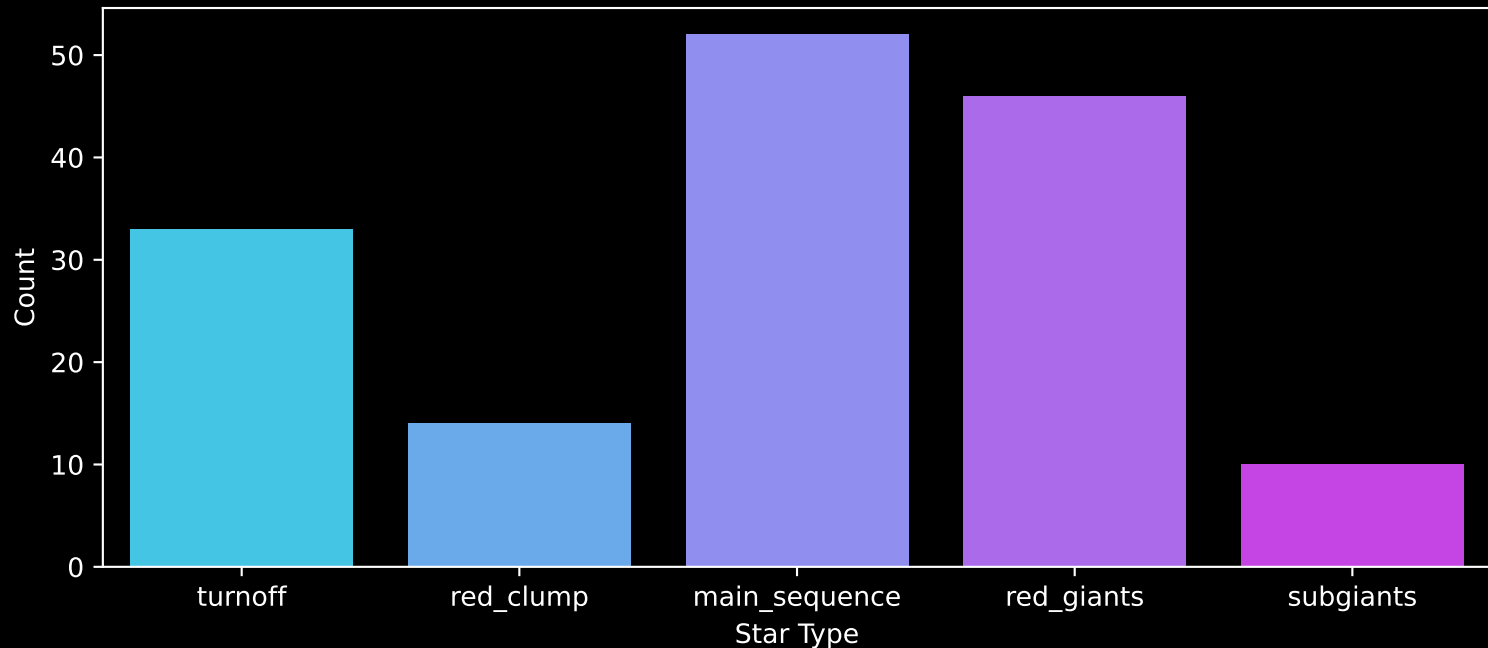
APOGEE DR17 Field: [276-25-O] Count plot of Star Type
