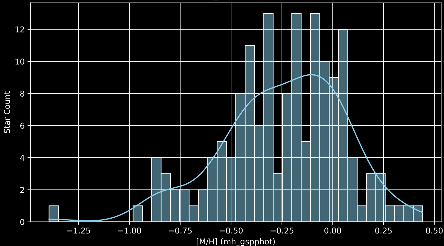
APOGEE DR17 Field: [276-25-O [M/H] (mh_gspphot) (n= 155)
