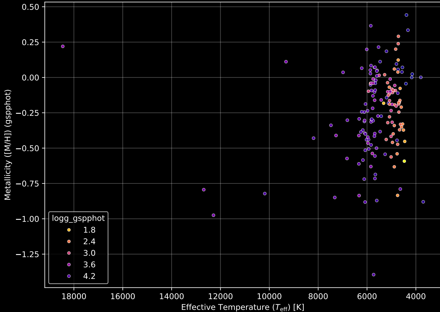
APOGEE DR17 Field: [276-25-O] Stellar Population Parameters (n= 155)
