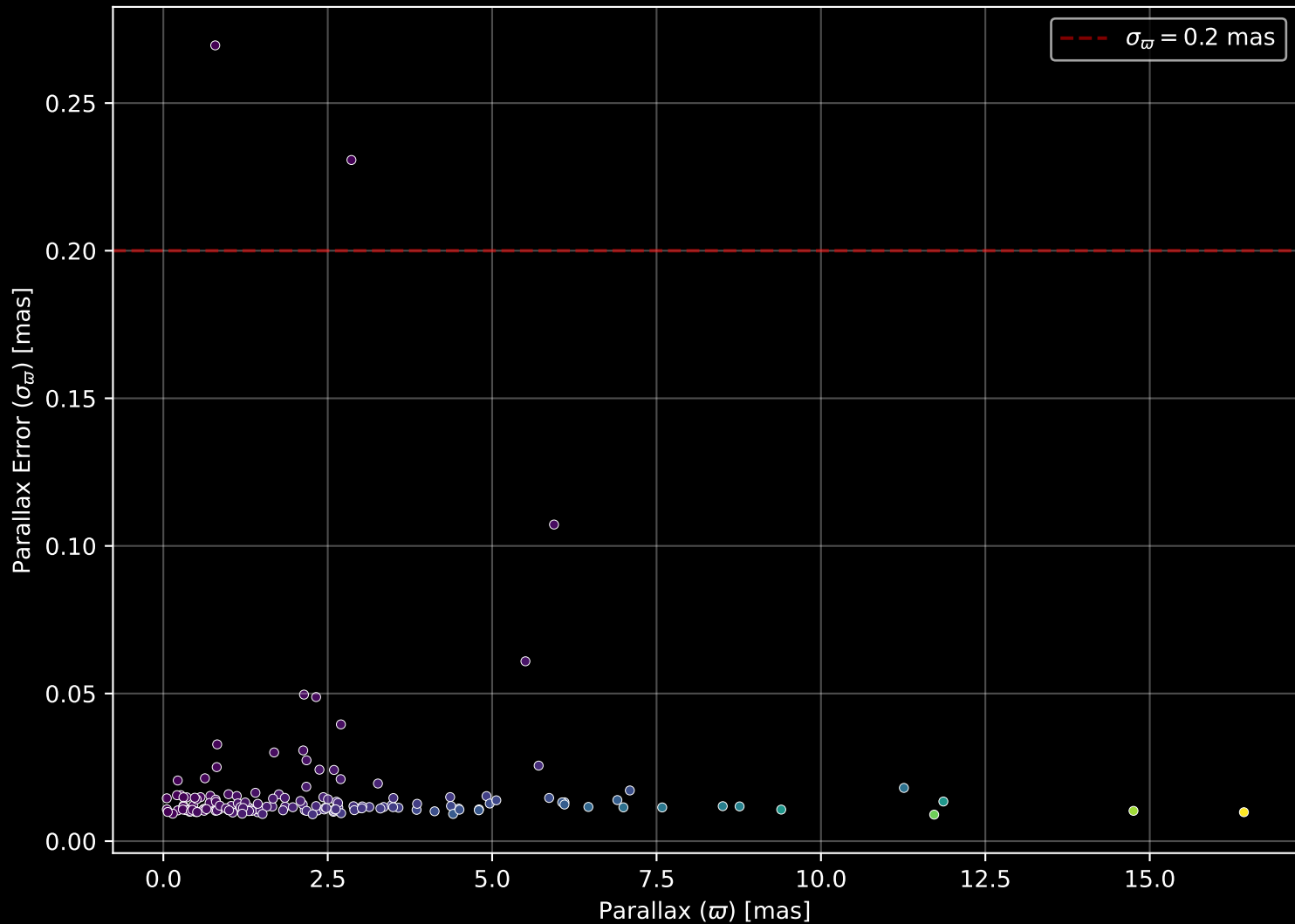
APOGEE DR17 Field: [276-25-O] Parallax Quality (n= 155)
