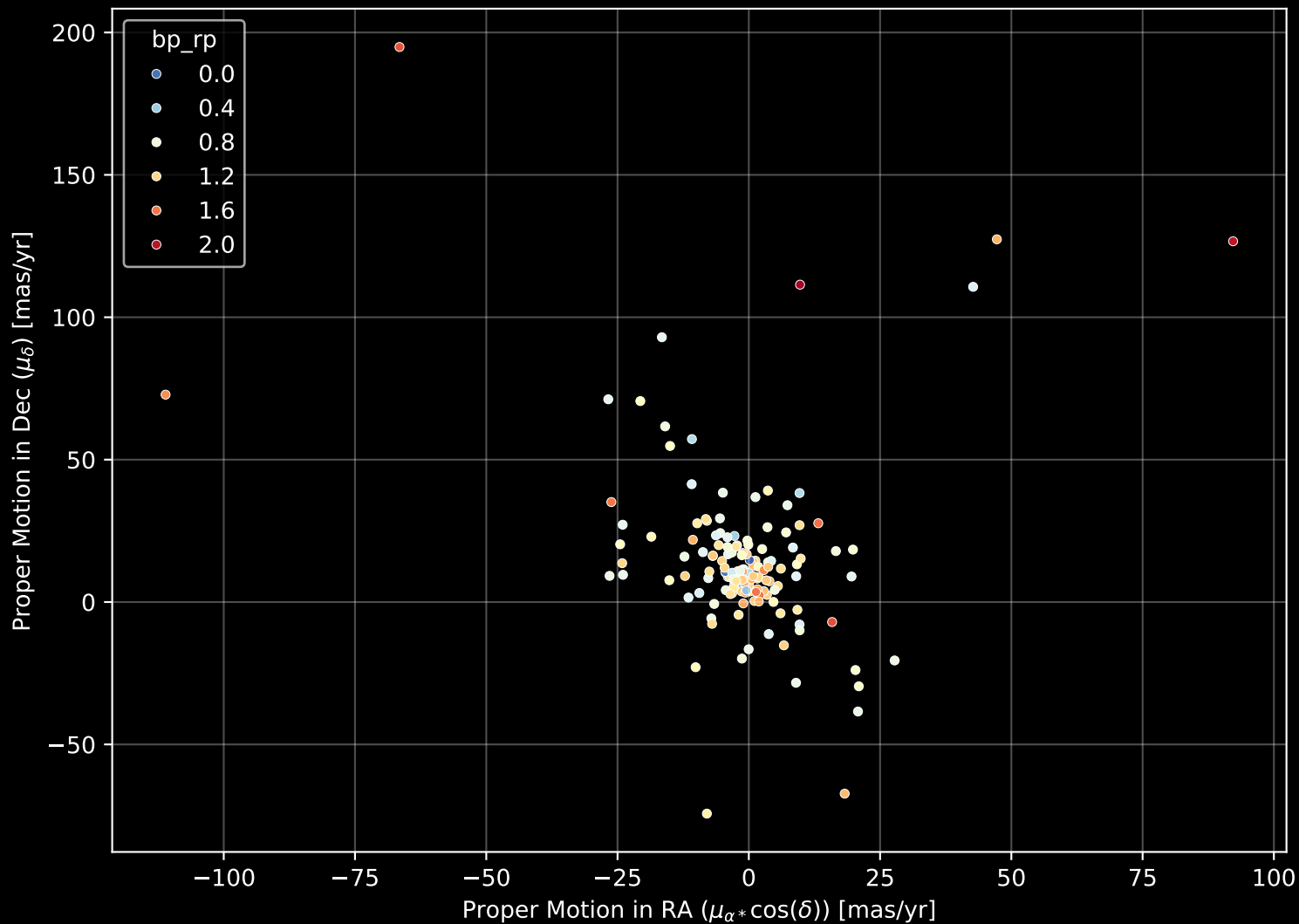
APOGEE DR17 Field: [276-25-O] Proper Motion Diagram (n= 155)
