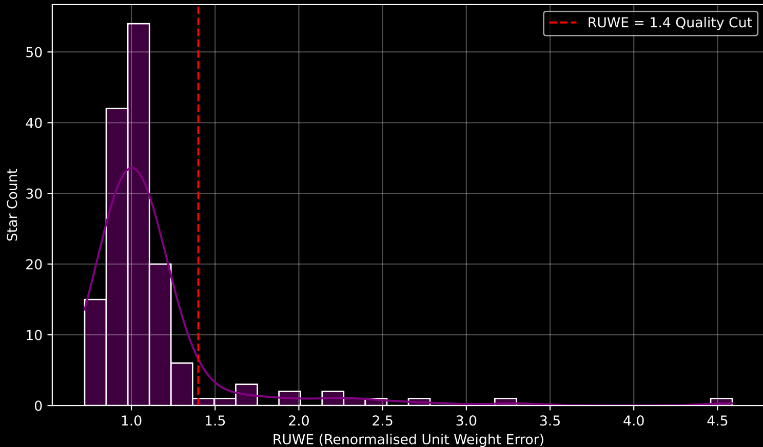
GAPOGEE DR17 Field [276-25-O] RUWE Distribution (n= 151)
